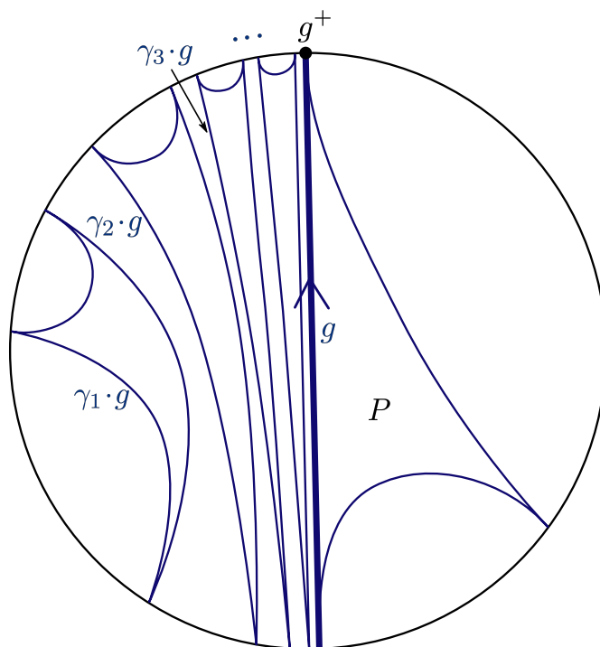
Figure 6.2.: If the leaf g bounding P is non-isolated and its endpoint g^+ is not a fixed point of an element in \pi_1(S) , then there exists a sequence (\gamma_n)_{n \in \mathbb{N}} such that the sequence of geodesics (\gamma_n \cdot g)_{n \in \mathbb{N}} converges to g .
