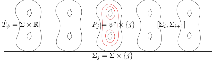
FIGURE 2. Infinite cyclic covering.
